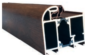
Ościeznica TERMO do PREMIUM i EXPERT 64
